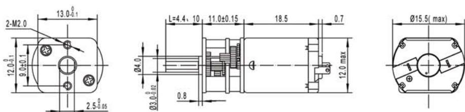
Gear Motor Dimensions (mm)
