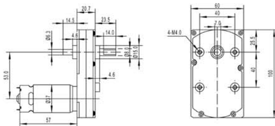
Gear Motor Dimensions (mm)
